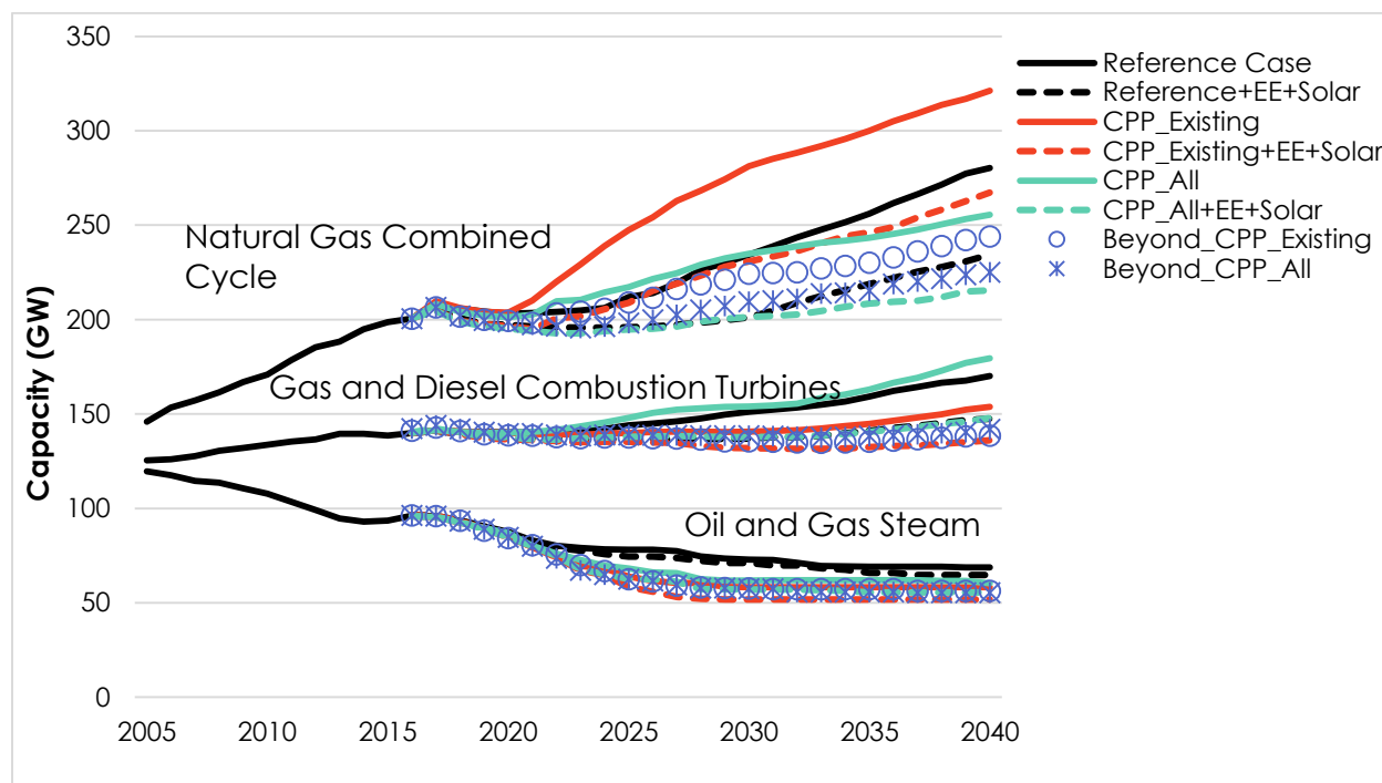
Figure 4.8. Capacity of Natural Gas (and Oil and Diesel) Generators (in GW)
